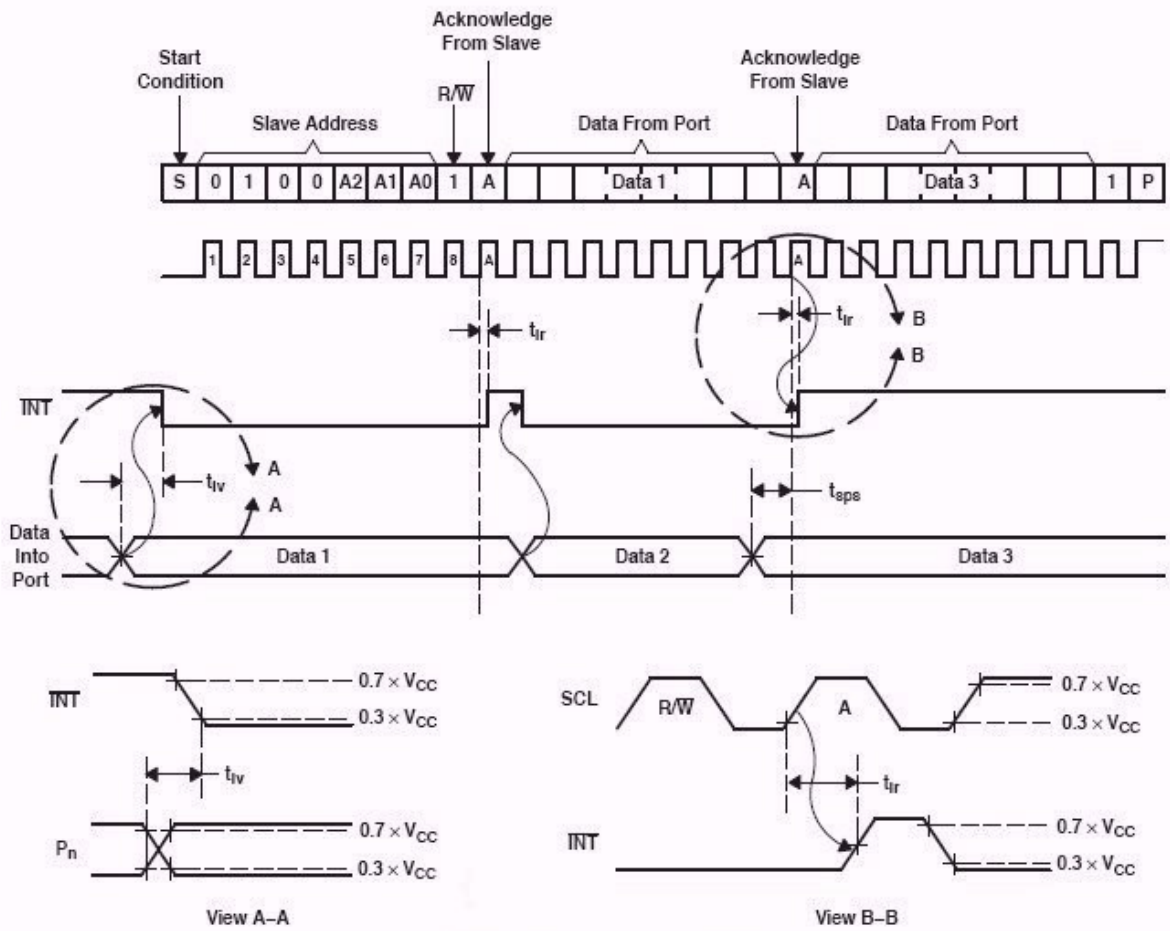
Figure 15. Interrupt Voltage Waveforms
